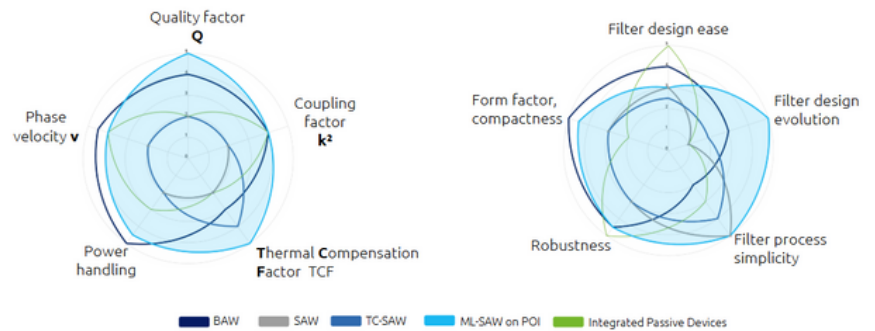
RF filter Figures of Merit comparison
